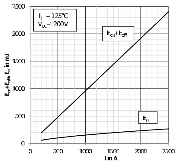
Fig. 4: Typical energy losses E = f(I_C, V_{CC})
